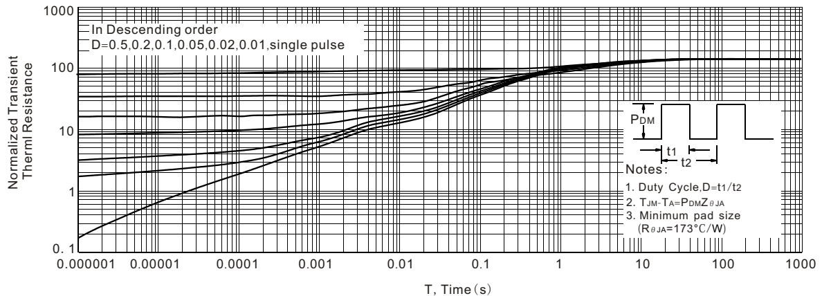
Figure 10. Thermal Response
